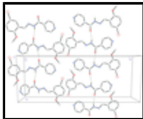
Fig. 2. The packing diagram of the title compound, viewed along the c axis. Hydrogen bonds are shown as dashed lines.
